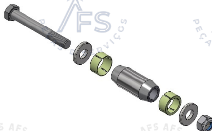
5234363 PINO EXPANDER Ø35
