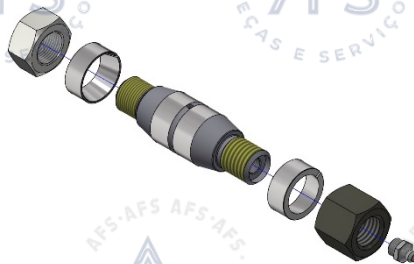
5072182 (5047010) PINO EXPANDER
